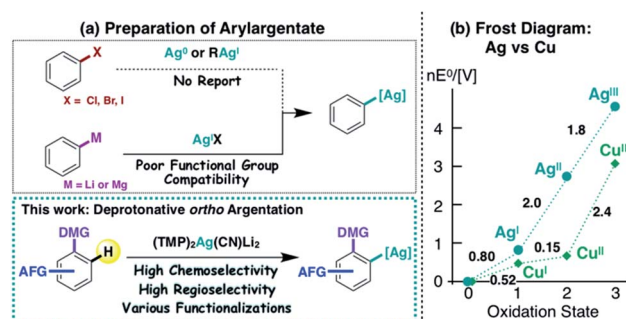
Fig. 1 (a) Preparative strategies for arylargentates, and (b) comparison of electrochemical properties of copper and silver.
