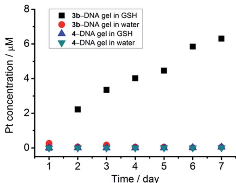
Fig. 7 Platinum release from [Pt(bzimpy)Cl] + -DNA hydrogels by incubation of the hydrogels in 10 mM GSH aqueous solution at room temperature.
