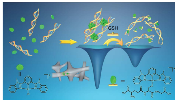
Scheme 3 Supramolecular system of [Pt(bzimpy)Cl] + and double-stranded DNA. The platinum(II) complexes stack into columnar phases and then non-covalently crosslink the DNA strands by electrostatic attractions to form hydrogels. In GSH aqueous solution, the ligand exchange reaction of the chloro ligand in [Pt(bzimpy)Cl] + with GSH endows the complexes with enhanced hydrophilicity, decreasing the planarity of the complexes, and turning off the metal-metal and π-π interactions at the crosslinking points, leading to energetically unfavorable hydrogel dissociation. The wells represent the qualitative energy profile of the system.
