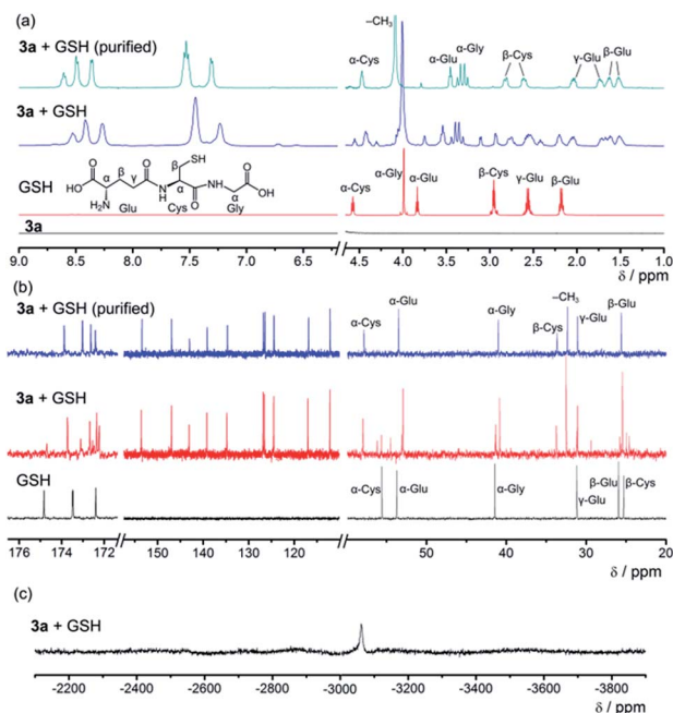
Fig. 8 (a) 1 H NMR, (b) 13 C{ 1 H} NMR and (c) 195 Pt{ 1 H} NMR spectra of the 3a -GSH reaction system in D 2 O.
