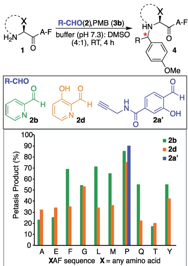
Fig. 4 Peptide modification with Petasis reaction. Peptides with sequence XAF, where X represents a variable amino acid were screened for reaction with PMB 3b and a variety of aldehydes 2b, 2d and water-soluble SAL analogue 2a'. % conversion to Petasis products were determined by LC/MS. Reaction conditions: XAF (12–17 mM), RCHO 2 (1.5 equiv. 18–25.5 mM), PMB 3b (8 equiv. 96–136 mM) in 25 mM buffer (pH 7.3) : DMSO (4 : 1) and 37 °C. The samples were incubated for 4 h.
