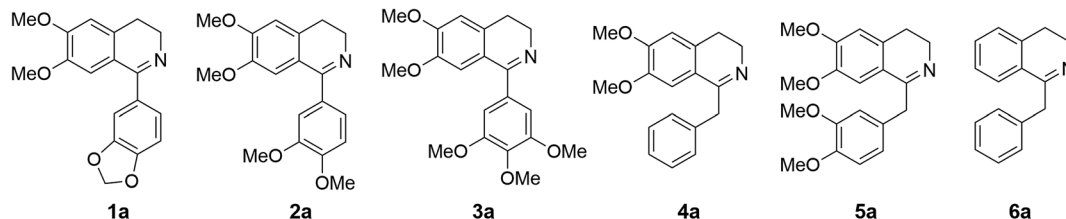
Scheme 3 DHIQ substrates prepared and used in this study.
