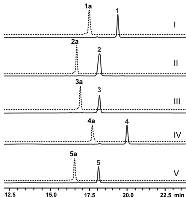
Fig. 2 Production of THIQs 1–5 in the IRED-based biosynthetic systems. The retention time of the precursors 1a – 5a is indicated by the dashed lines. Samples from the biosynthetic systems are indicated by the solid lines in dark blue. (I) Biosynthesis of 1 from 1a by E. coli with F190M–W191F + GDH + CNMT; (II) biosynthesis of 2 from 2a by the crude enzymes F190L–W191F + GDH and E. coli with CNMT; (III) biosynthesis of 3 from 3a by the crude enzymes F190L–W191F + GDH and E. coli with CNMT; (IV) biosynthesis of 4 from 4a by E. coli with F190M–W191F + GDH + CNMT; (V) biosynthesis of 5 from 5a by E. coli with F190M–W191F + GDH + CNMT.
