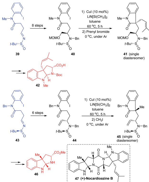
Scheme 10 Synthetic route towards (+)-nocardiozine B.
