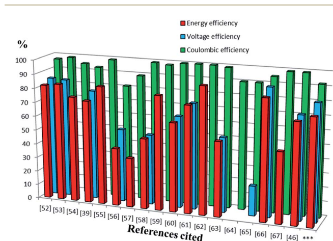
Fig. 7 The bars represent the CE, EE and VE of redox flow battery systems containing iron in their electrolyte system reported in the literature. Sequence of references followed by electrolyte system with concentration of active redox species, cell voltage (V) and volumetric capacity ( \text{Ah L}^{-1} ) are as follows: 52 1.5 \text{ M Fe}^{3+}/\text{Fe}^{2+}/1.5 \text{ M V}^{3+}/\text{V}^{2+} (1.02 V, 18 \text{ A h L}^{-1} ), 53 0.1 \text{ M Fc1N112-TFSI}/\text{Fe}(\text{acac})_3 (1.34 V, 2.47 \text{ A h L}^{-1} ), 54 \text{Fe}_3\text{O}_4/\text{Fe}/0.2 \text{ M Fe}(\text{CN})_6^{3-}/\text{Fe}(\text{CN})_6^{4-} (1.2 V, 0.00065 \text{ A h L}^{-1} ), 39 0.2 \text{ M } [\text{Fe}(\text{TEOA})\text{OH}]^{-}/[\text{Fe}(\text{TEOA})\text{OH}]^{2-}/0.2 \text{ M Fe}(\text{CN})_6^{3-}/\text{Fe}(\text{CN})_6^{4-} (1.34 V, 4 \text{ A h L}^{-1} ), 55 0.5 \text{ M 2,6-DHAQ dipotassium salt}/0.4 \text{ M K}_4\text{Fe}(\text{CN})_6 (1.20 V), 56 0.1 \text{ M FeSO}_4 + 0.5 \text{ M NaCl}/0.1 \text{ M Fe}(\text{acac})_3 , 57 1.5 \text{ M Fe}^{2+}/\text{Fe}^{3+}/1.8 \text{ M Cu}^{+}/\text{Cu}^0 (0.25 V), 58 0.5 \text{ M alloxazine-COOH}/0.4 \text{ M Fe}(\text{CN})_6^{4-} (1.3 V, 24 \text{ A h L}^{-1} ), 59 0.3 \text{ M 2,7-AQDS}/0.1 \text{ M Fe}(\text{CN})_6^{4-} (0.76 V, 17.8 \text{ A h L}^{-1} ), 60 0.5 \text{ M ACA}/0.4 \text{ M Fe}(\text{CN})_6^{4-} + 40 \text{ mM Fe}(\text{CN})_6^{3-} (1.13 V), 61 0.5 \text{ M } (\text{NH}_4)_4[\text{Fe}(\text{CN})_6]/0.5 \text{ M } (\text{SPR})_2\text{V} (0.82 V, 10 \text{ A h L}^{-1} ), 62 0.1 \text{ M bislawsonne}/0.2 \text{ M K}_4\text{Fe}(\text{CN})_6/0.02 \text{ M K}_3\text{Fe}(\text{CN})_6 (1.05 V), 63 0.1 \text{ M Cr}(\text{acac})_3/0.1 \text{ M Fe}(\text{acac}) (1.2 V, 0.67 \text{ A h L}^{-1} ), 64 0.01 \text{ M Co}(\text{phen})_3/0.01 \text{ M Fe}(\text{phen})_3 (2.1 V, 0.10 \text{ A h L}^{-1} ), 65 0.2 \text{ M } [\text{Co}(\text{bpy})_3]\text{Tf}_2/0.2 \text{ M } [\text{Fe}(\text{bpy})_3]\text{Tf}_2 (2.0 V), 66 0.1 \text{ M FeCp}_2\text{PF}_6/0.1 \text{ M CoCp}_2 (1.7 V, 2.5 \text{ A h L}^{-1} ), 67 0.20 \text{ M K}_4\text{Fe}(\text{CN})_6 , 0.08 \text{ M K}_3\text{Fe}(\text{CN})_6/0.1 \text{ M 2,6-DBEAQ} (1.05 V), 46 0.5 \text{ M Co(II)-mTEA}/0.25 \text{ M Fe(III)-TEA} + 0.5 \text{ M Fe(II)-TEA} (0.93 V) and ***this work.
