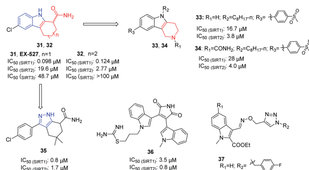
Fig. 6 Chemical structures of indole-based SIRT2 inhibitors and their inhibitory activity data on SIRT2 by isotope labelling, 49 Sirt-Glo™ assay kit 50 or fluorescence-based assays. 51
