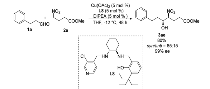
Scheme 16 Asymmetric syn -selective Henry reaction catalyzed by C 1 -symmetrical amino-alcohol ligand L8.
