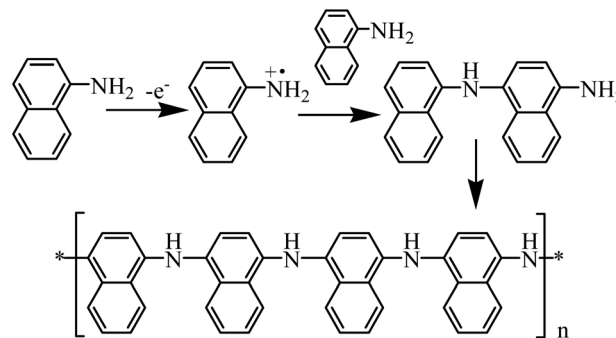
Scheme 4 Poly-1-naphthylamine.
