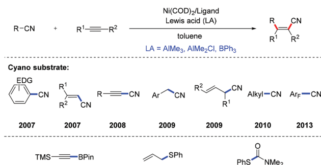
Scheme 4 Ni-Catalyzed carbocyanation, alkynylboration, thioallylation and thiocarbamylation of alkynes.
