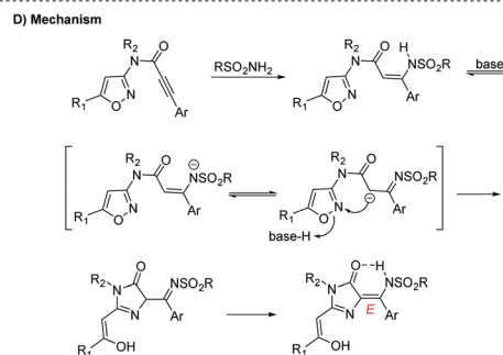
Scheme 28 Cai and co-workers' synthesis of imidazol-4-ones via rearrangement of isoxazoles.
