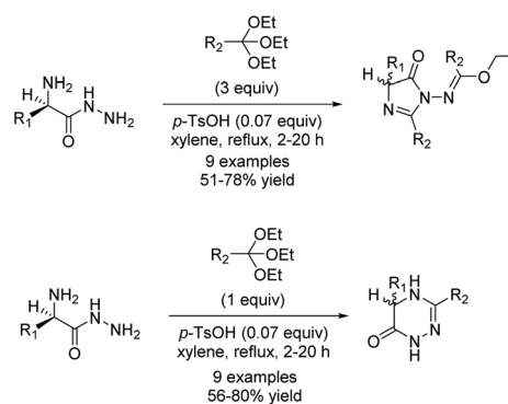
Scheme 9 Jasiak and co-workers' synthesis of imidazol-4-ones from optically active \alpha -aminocarboxylic acid hydrazides.
