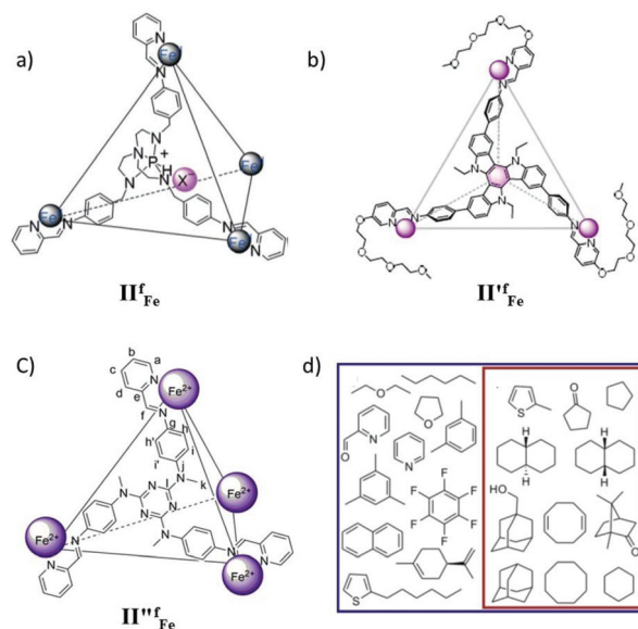
Fig. 6 Representation of tetrahedral cages: (a) \text{II}^{\text{III}}_{\text{Fe}} , (b) \text{II}^{\text{II}}_{\text{Fe}} , (c) \text{II}^{\text{II}}_{\text{Fe}} and (d) guest molecules encapsulated in cage \text{II}^{\text{II}}_{\text{Fe}} , in \text{D}_2\text{O} all molecules whereas there is a subset in \text{CD}_3\text{CN} . Reproduced with permission from ref. 51–53. Copyright 2018, John Wiley & Sons, Ltd; 2019, and 2014, the American Chemical Society.
