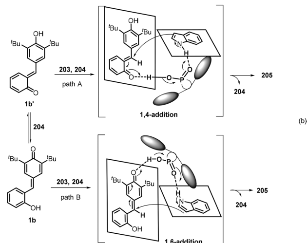
Scheme 42 Asymmetric addition of indoles to p -QMs.
