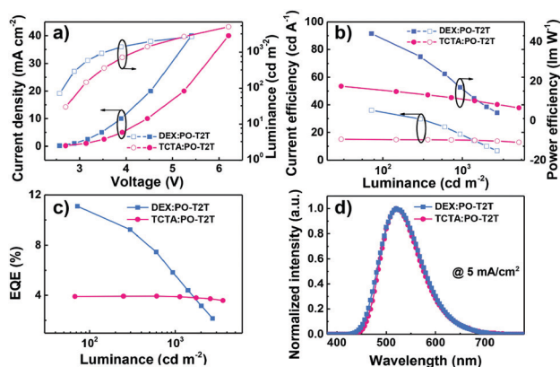
Fig. 4 (a) J – V – L plots, (b) CE–luminance–PE plots, (c) EQE–luminance plots, and (d) EL (at 5 \text{mA cm}^{-2} ) spectra of DEX:PO-T2T and TCTA:PO-T2T exciplex-based devices.
