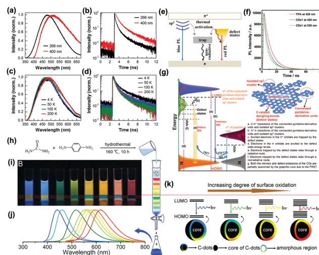
Fig. 4 (a) PL spectra of GQDs obtained by thermal deoxidization of GO sheets and (b) PL decay curves of ensemble GQDs excited at 266 and 400 nm by pulsed laser. (c) PL spectra and (d) PL decay curves of ensemble GQDs measured at four temperatures with pulsed laser excitation at 266 nm. (e) Energy level structures on GQDs; energy level structures to explain the optical behaviors of photoexcited electrons in both GO sheets and GQDs. 84 (Reprinted with permission from the American Chemical Society, Copyright 2013.) (f) PL decays of free TPA (3,5-dihydro-5-oxo-2H-thiazolo[3,2-a]pyridine-3,7-dicarboxylic acid) and CDs synthesized by thermal treating a mixture of citric acid and amino group-containing molecules at 345 nm laser excitation. (g) Representation of the PL mechanism of CDs. 85 (Reprinted with permission from Elsevier Ltd, Copyright 2017.) (h) One-pot synthesis and purification route for CDs with distinct fluorescence characteristics. (i) Eight CDs samples under 365 nm UV light. (j) Corresponding PL emission spectra of the eight samples, with maxima at 440, 458, 517, 553, 566, 580, 594, and 625 nm. (k) Model for the tunable PL of CDs with different degrees of oxidation. 86 (Reprinted with permission from the American Chemical Society, Copyright 2016.).
