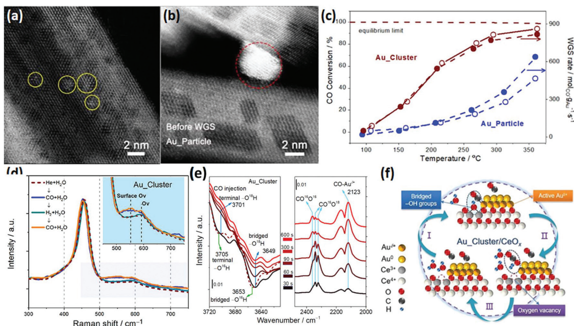
Fig. 14 High-angle annular dark-field scanning transmission electron microscopy (HAADF-STEM) images of (a) Au-cluster/CeO x and (b) Au-particle/CeO x catalyst. (c) Catalytic activity for the WGSR by the Au-cluster/CeO x and Au-particle/CeO x catalysts. (d) In situ Raman spectra of Au-cluster/CeO x under different atmospheres at 150 °C. (e) In situ time-sequencing IR spectra of Au-cluster/CeO x under CO injection with isotope prelabeled using H 2 O. 18 (f) Schematic illustration of the reaction mechanism of Au-cluster/CeO x catalyst for the WGS. Adapted with permission from ref. 15. Copyright 2019, American Chemical Society.
