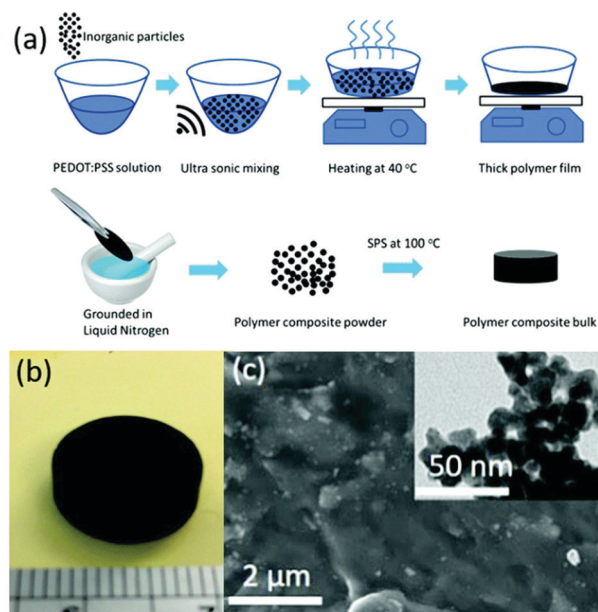
Fig. 5 (a) Process used to synthesize bulk polymers. (b) Photograph of a polymer bulk sample after applying SPS. (c) SEM image of the polymer bulk with an inset showing a TEM image of \text{Cu}_2\text{SnSe}_3 nanoparticles. (Reproduced from ref. 56 with permission from The Royal Society of Chemistry.).
