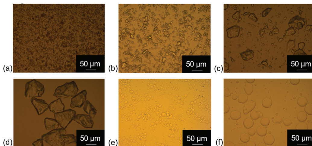
Fig. 1 Light microscopy images of powder fractions used for the preparation of model chocolate samples, sugar and quartz beads model systems in sunflower oil. (a) Bensdorp Red-D-light cocoa powder; (b) fine sugar fraction; (c) medium sugar fraction; (d) coarse sugar fraction; (e) fine quartz beads fraction; (f) coarse quartz beads fraction.
