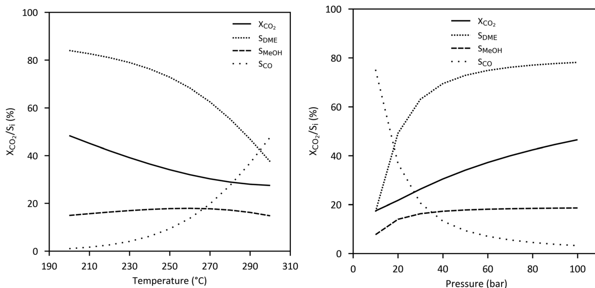
Fig. 13 Equilibrium conversion of \text{CO}_2 ( = [\text{CO}_{2,\text{in}} - \text{CO}_{2,\text{out}}]/\text{CO}_{2,\text{in}} ) and selectivity of DME, methanol and CO ( S_i = i/[\text{CO}_{2,\text{in}} - \text{CO}_{2,\text{out}}] , with i = 2 \times \text{DME/MeOH/CO} , based on amount of C-atoms) dependent on (a) temperature and (b) pressure ( \text{H}_2 : \text{CO}_2 = 3 : 1 , based on Aspen Plus Simulation).
