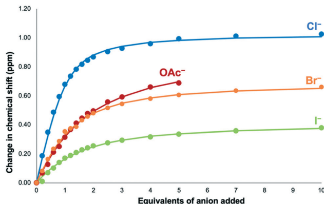
Fig. 3 ^1\text{H} NMR binding curve for addition of TBA-Cl, TBA-Br, TBA-I and TBA-OAc to 5\cdot(\text{PF}_6)_3 , showing the change in chemical shift of \text{H}_4 (9:1 \text{CD}_3\text{CN} : d^6\text{-DMSO} , 298 K). Dots represent the observed points and the line represents 1:1 binding isotherms fitted using Bindfit. 41 Precipitation was observed after addition of five equivalents of TBA-OAc.
