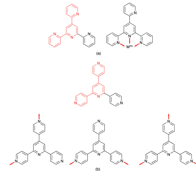
Scheme 2 Examples of tpy motifs as units within quaterpyridines. (a) 4'-(Pyridin-2-yl)-2,2':6',2''-tpy contains a 2,2':4',2''-tpy unit (in red) but typically binds metal ions as a bis(chelate). (b) 4'-(Pyridin-4-yl)-4,2':6',4''-tpy contains a 4,2':4',4''-tpy unit (in red); three possible ditopic modes of bonding of 4'-(pyridin-4-yl)-4,2':6',4''-tpy represented in the CSD by refcode entries AGUPUO (left), QOTREY (middle) and RIGPII (right).
