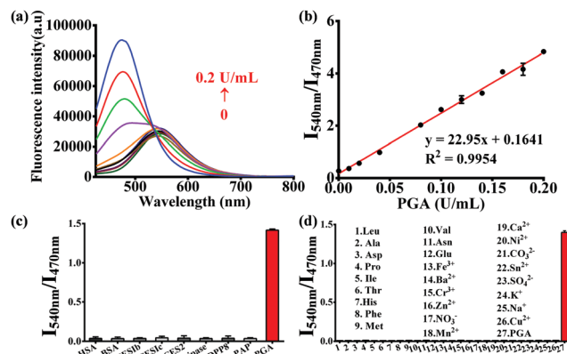
Fig. 1 (a) Fluorescence spectra of PNA (10 \mu\text{M} ) upon addition of increasing concentrations of PGA (0–0.2 \text{U mL}^{-1} ). (b) Linear relationship between the fluorescence ratio ( I_{540\text{nm}}/I_{470\text{nm}} ) and PGA concentration. Fluorescence intensity ratio ( I_{540\text{nm}}/I_{470\text{nm}} ) of PNA upon addition of various enzymes and proteins (c), ions and amino acids (d). (PGA 0.05 \text{U mL}^{-1} , PBS : acetonitrile 2 : 1, v/v, \lambda_{\text{ex}} 400 nm).
