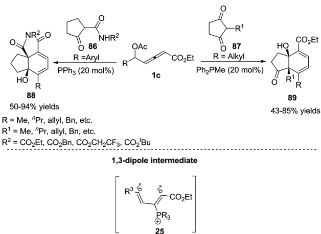
Scheme 28 Phosphine-catalyzed (4+2) annulations of \delta -acetoxy allenates and ketones.
