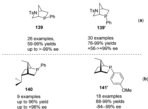
Scheme 45 Hydroxyproline-derived pseudoeantiomeric[2.2.1]bicyclic phosphines: asymmetric synthesis of (+)- and (-)-pyrrolines.
