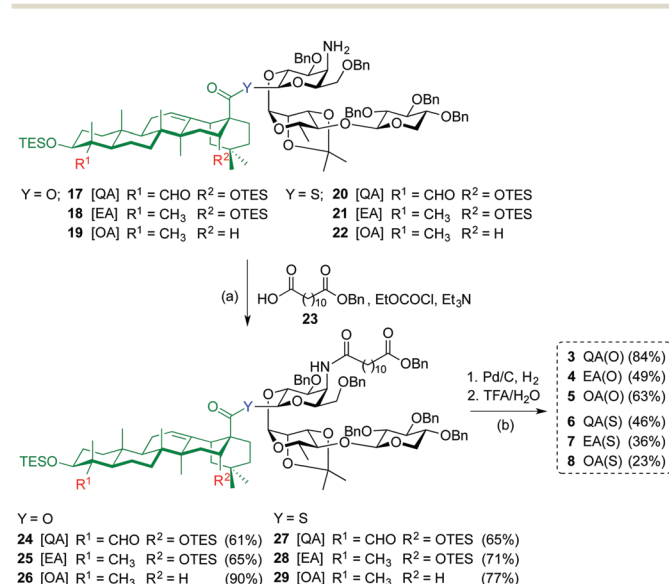
Scheme 2 Reagent and conditions: (a) \text{EtOCOC(=O)H} , \text{Et}_3\text{N} , THF, 0 °C to r.t., 4 h, 61% (for 24 ), 65% (for 25 ), 90% (for 26 ); 65% (for 27 ), 71% (for 28 ), and 77% (for 29 ); (b) 1: Pd/C, \text{H}_2 (1 atm), \text{EtOH}/\text{THF} 1 : 1, r.t., 16 h (for 24–26 ); 20 min (for 27–29 ); 2: TFA/ \text{H}_2\text{O} 3 : 1, 0 °C, 1 h, 84% (for 3 ), 49% (for 4 ), 63% (for 5 ); 46% (for 6 ), 36% (for 7 ), and 23% (for 8 ).
