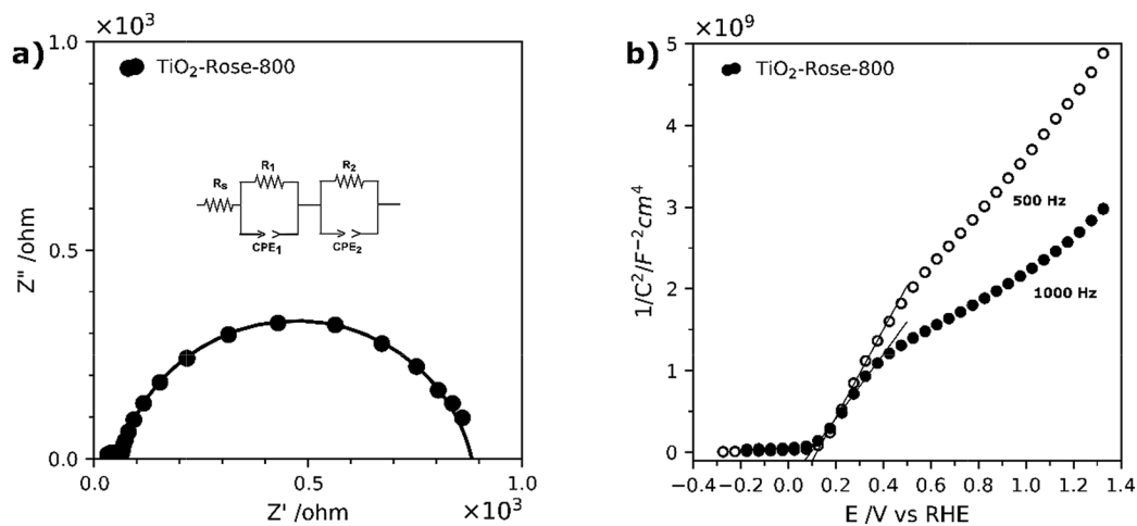
Fig. 10 (a) Nyquist plots of \text{TiO}_2 -Rose-800 at the open circuit potential (OCP) of the cell under 1 sun illumination (AM 1.5G, 100 \text{ mW cm}^{-2} ). (b) Mott-Schottky plots at a fixed frequency of 500 Hz and 1000 Hz of \text{TiO}_2 -Rose-800 in 1 M KOH (pH = 13.6).
