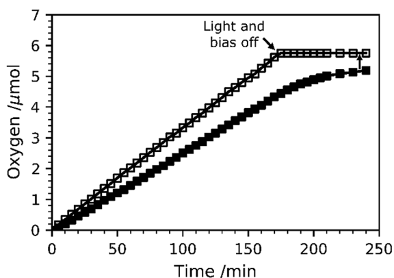
Fig. 11 Amount of \text{O}_2 gas evolved at 1.23 V_{\text{RHE}} under simulated sunlight (AM 1.5G, 100 \text{ mW cm}^{-2} ). The amount of \text{O}_2 quantified with a fluorescence probe is represented by solid markers, whereas the theoretical amount of \text{O}_2 calculated assuming a 100% faradaic efficiency is shown with empty markers.
