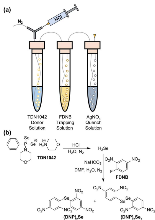
Fig. 5 (a) Experimental setup for volatilization and trapping of \text{H}_2\text{Se} with FDNB. (b) General reaction pathways for (DNP) 2 Se and (DNP) 2 Se 2 formation.
