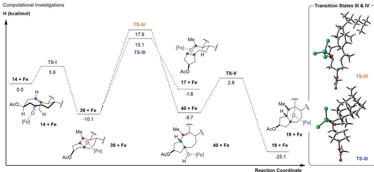
Fig. 4 Reaction path for transannular carbonyl-olefin metathesis and the formation of furans from intermediate oxetanes 39.
