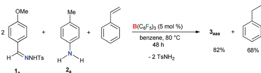
Scheme 4 Kinetic and mechanistic studies for the synthesis of 1,2,4-triazole.
