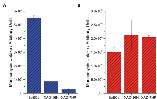
Fig. 3 Relative uptake of marinomycin A ( 1 ) by 50 mg of XAD 7HP, XAD 16N and SpECs. (A) Uptake of marinomycin A ( 1 ) from a crude culture broth. Relative quantification by mass LC-MS by integration of the XIC between 997.5 and 997.6 Da. (B) Uptake of marinomycin A ( 1 ) from aliquots of the purified compound in water. Concentration ( \mu\text{M} ) of purified marinomycin A ( 1 ) taken up by 50 mg of XAD 7HP, XAD 16N and SpECs.
