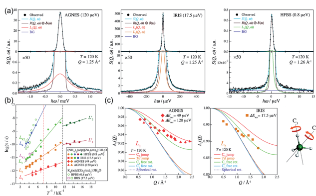
Fig. 20 (a) QENS profiles of (\text{NH}_4)_2(\text{adp})[\text{Zn}_2(\text{ox})_3] \cdot 3\text{H}_2\text{O} obtained by using AGNES, IRIS, and HFBS spectrometers. (b) Arrhenius plot for the relaxation times of (\text{NH}_4)_2(\text{adp})[\text{Zn}_2(\text{ox})_3] \cdot 3\text{H}_2\text{O} (filled symbols) and \text{K}_2(\text{adp})[\text{Zn}_2(\text{ox})_3] \cdot 3\text{H}_2\text{O} (open symbols) at Q_{\text{av}} = 1.25 \text{ \AA}^{-1} . (c) EISF of (\text{NH}_4)_2(\text{adp})[\text{Zn}_2(\text{ox})_3] \cdot 3\text{H}_2\text{O} for the L_1 mode measured by AGNES (left) and the L_2 mode measured by IRIS (right). Solid curves represent the calculated EISF based on several model functions. Reproduced from ref. 77 with permission from Royal Society of Chemistry, Copyright 2014.
