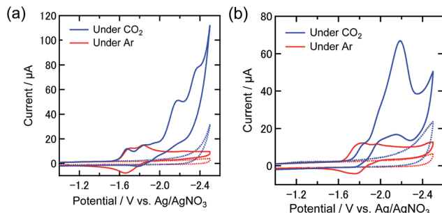
Fig. 2 CVs of the Re(I) complex(es) (total 0.5 mM) (a) in DMF and (b) in the DMF-TEOA (5 : 1 v/v) mixed solution, containing \text{Et}_4\text{NBF}_4 (0.1 M) as the supporting electrolyte at a sweep rate of 200 \text{ mV s}^{-1} . Blue and red lines show the CVs under \text{CO}_2 and Ar, respectively. Dotted lines indicate CVs for the corresponding solutions without the Re(I) complex. A glassy carbon electrode (diameter: 3 mm), an Ag/AgNO 3 (10 mM) electrode and a Pt wire were used as working, reference, and counter electrodes, respectively.
