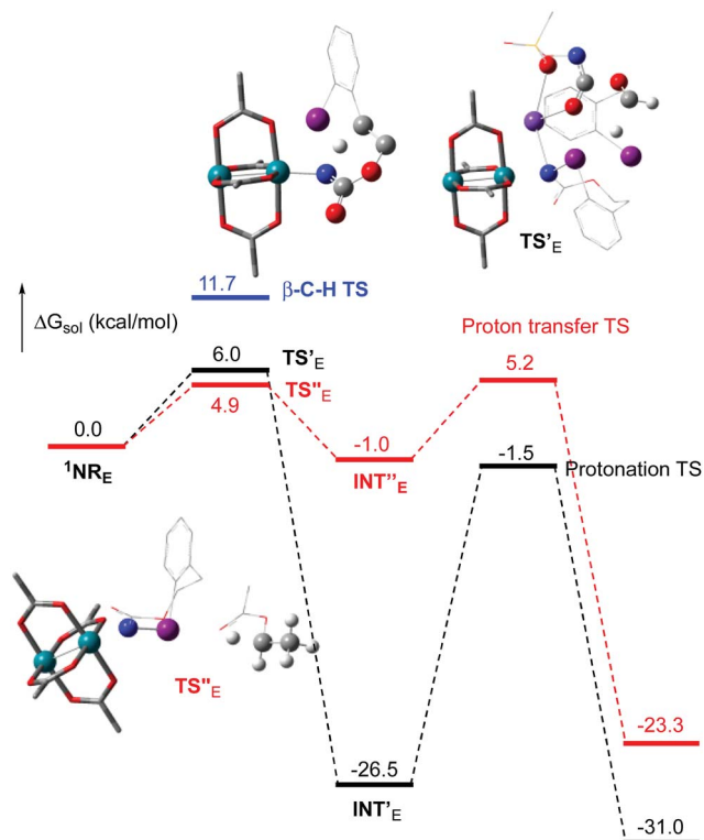
Fig. 12 Calculated free energy profile for the reactivity of \text{NR}_\text{E} at the PBE/BS2 level of theory (the relative free energies ( \Delta G_{\text{sol}} , kcal mol -1 ) in ethyl acetate are provided). (Different atom styles are used for clarity.)
