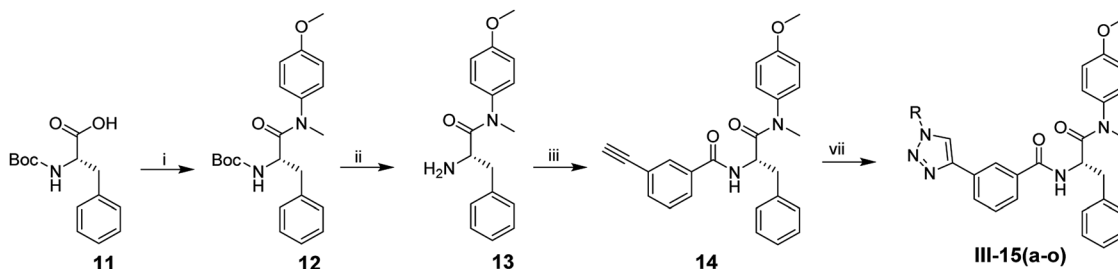
Scheme 3 Reagents and conditions used to synthesize III-15(a–o) . (i) 4-methoxy- N -methylaniline, PyBop, DIEA, CH 2 Cl 2 , r.t., 8–10 h; (ii): CF 3 COOH; CH 2 Cl 2 , r.t., 5–6 h; (iii) 3-ethynylbenzoic acid, HATU, DIEA, CH 2 Cl 2 , r.t., 10 h; (vii): azide substituents; CuSO 4 ·5H 2 O, VcNa, THF/H 2 O (v : v = 1 : 1), 30–60 °C, 4–6 h.
