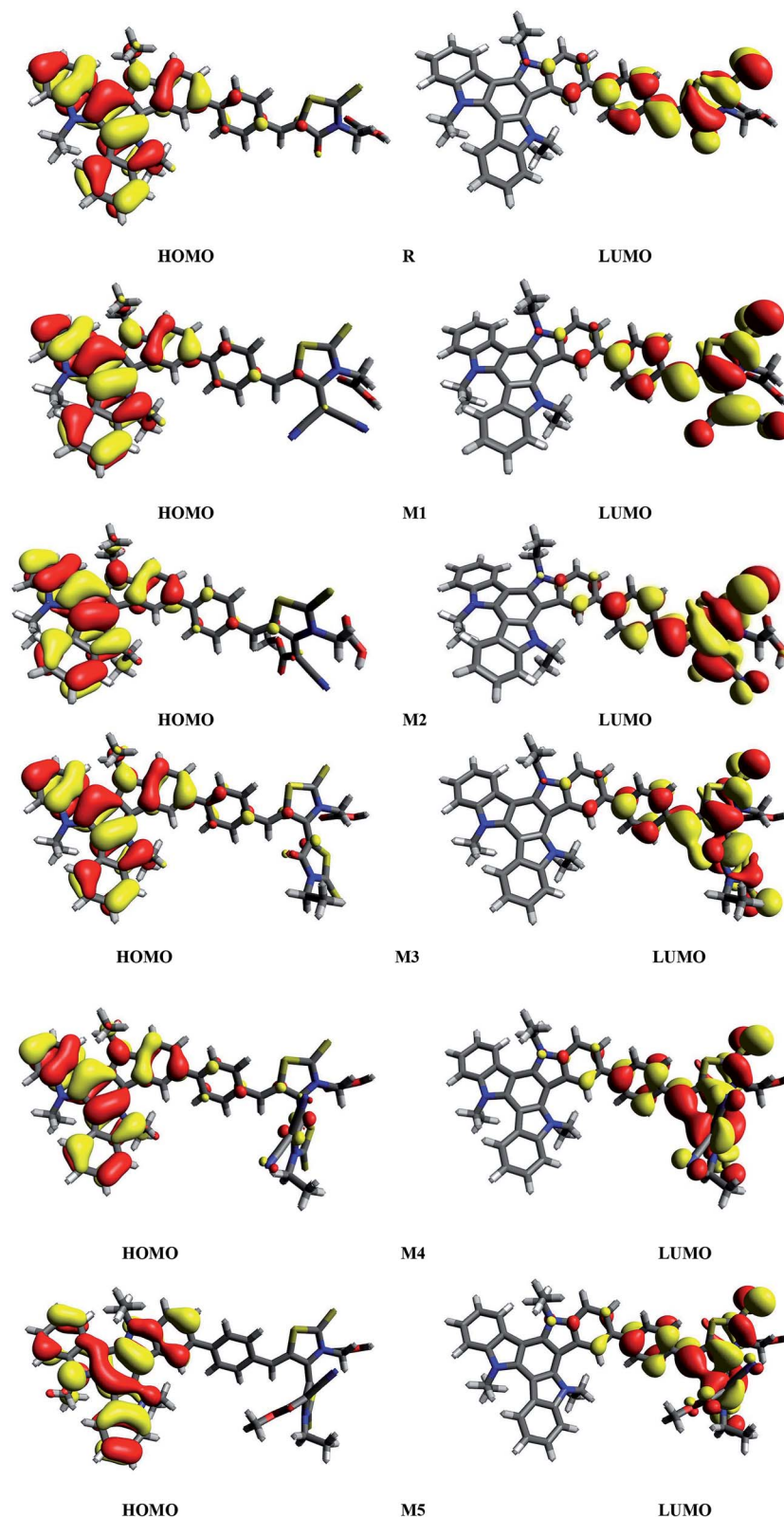
Fig. 4 HOMO and LUMOs of reference R and designed molecules ( M1 – M5 ) at B3LYP/6311G(d,p) level of theory.
