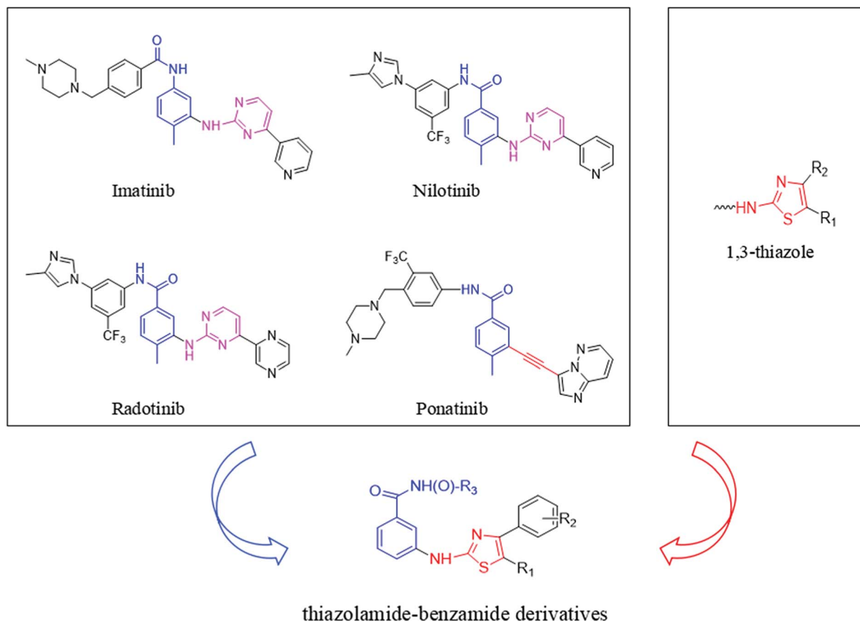
Fig. 1 Design of thiazolamide-benzamide derivatives as novel Bcr-Abl inhibitors.
