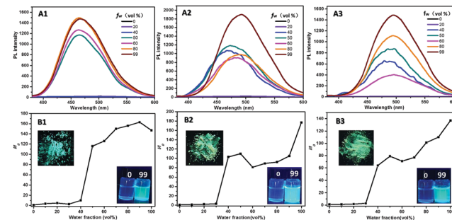
Fig. 3 Fluorescent spectra of TPE-L-Glu, cis -TPE-L-DGlu and trans -TPE-L-DGlu in THF/water mixed solvents with different f_w (A1–A3); plot of I_{00} values versus f_w (B1–B3), where I_0 represents the emission intensity in THF. Concentration: 1 \times 10^{-5} M; excitation wavelength: 340 nm. Inset: Photographs of TPE-L-Glu, cis -TPE-L-DGlu and trans -TPE-L-DGlu in solid and THF/water mixtures with 0 and 99% f_w under 365 nm UV lamp.
