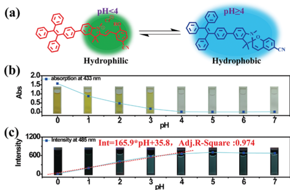
Fig. 2 (a) Illustration of switching between the ring-closed and protonated ring-open forms of TPE-Sp-CN at different pH values. (b) The plot of the absorption at 433 nm of the TPE-Sp-CN solutions (1 mL, 1 \times 10^{-4} M) treated with 0.2 mL water samples with different pH values (0 to 7). (c) The plot of the emission intensity of TPE-Sp-CN in acid solutions ( V_{\text{MeCN}} : V_{\text{acid water}} = 1 : 9 ) against pH (0 to 7).
