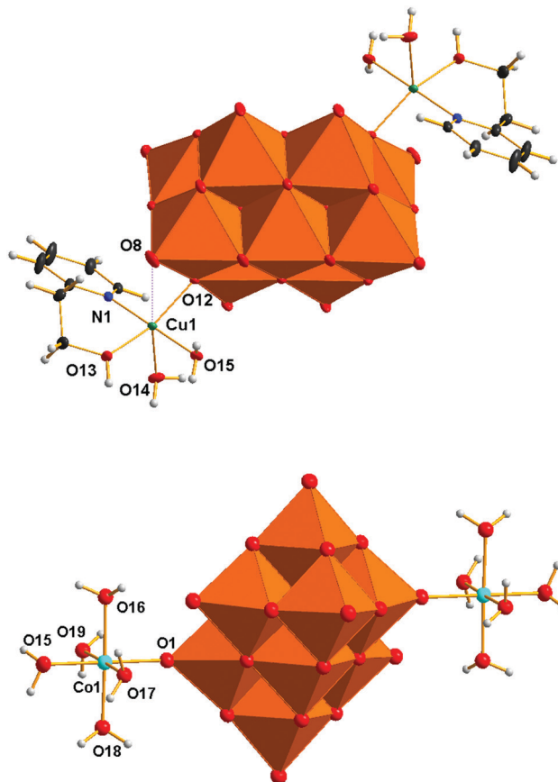
Fig. 1 Molecular structures of the anions [\{\text{Cu}(\text{H}_2\text{O})_2(2\text{-hep})\}_2\text{V}_{10}\text{O}_{28}]^{2-} ( \text{V}_{10}\text{Cu} ) and [\{\text{Co}(\text{H}_2\text{O})_5(2\text{-hep})\}_2\text{V}_{10}\text{O}_{28}]^{2-} ( \text{V}_{10}\text{Co} ) as revealed by X-ray crystallography showing atom labelling. Colour code: orange octahedra \{\text{VO}_6\} , green Cu, light blue Co, blue N, red O, black C, gray H. Ellipsoids are displayed at a 30% probability level.
