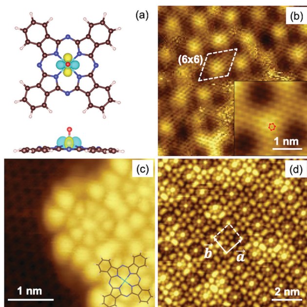
Fig. 1 (a) Molecular structure of VOPc. Color code: white, hydrogen; brown, carbon; blue, nitrogen; light blue, vanadium; red, oxygen. The isodensity of the surface ( \psi^2 = 0.06 \text{ e Bhor}^{-3} ), of the SOMO for \text{VOPc}@\text{Gr} is represented in yellow and light blue. (b) STM image of the \text{Gr}/\text{SiC}(0001) surface ( 10 \times 10 \text{ nm}^2 , -2 \text{ V} , filled states, 70 \text{ pA} , 1.8 \text{ K} ); the hexagonal atomic periodicity of the graphene layer is highlighted in the inset ( 2.5 \times 2.5 \text{ nm}^2 ); (c and d) STM images of the VOPc submonolayer deposited on \text{Gr}/\text{SiC}(0001) at two magnifications. (c) STM image 3.2 \times 3.2 \text{ nm}^2 ( 2 \text{ V} , filled states, 11 \text{ pA} , 1.7 \text{ K} ). The structure of a VOPc molecule is superimposed on the bottom-right corner as a visual guide. (d) STM image 10 \times 10 \text{ nm}^2 ( 2 \text{ V} , filled states, 11 \text{ pA} , 1.7 \text{ K} ). White arrows represent the unit-cell vectors of the molecular lattice ( \vec{a} and \vec{b} ).
