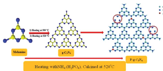
Scheme 2 Synthesis of P-g-C 3 N 4 by the calcination method.
