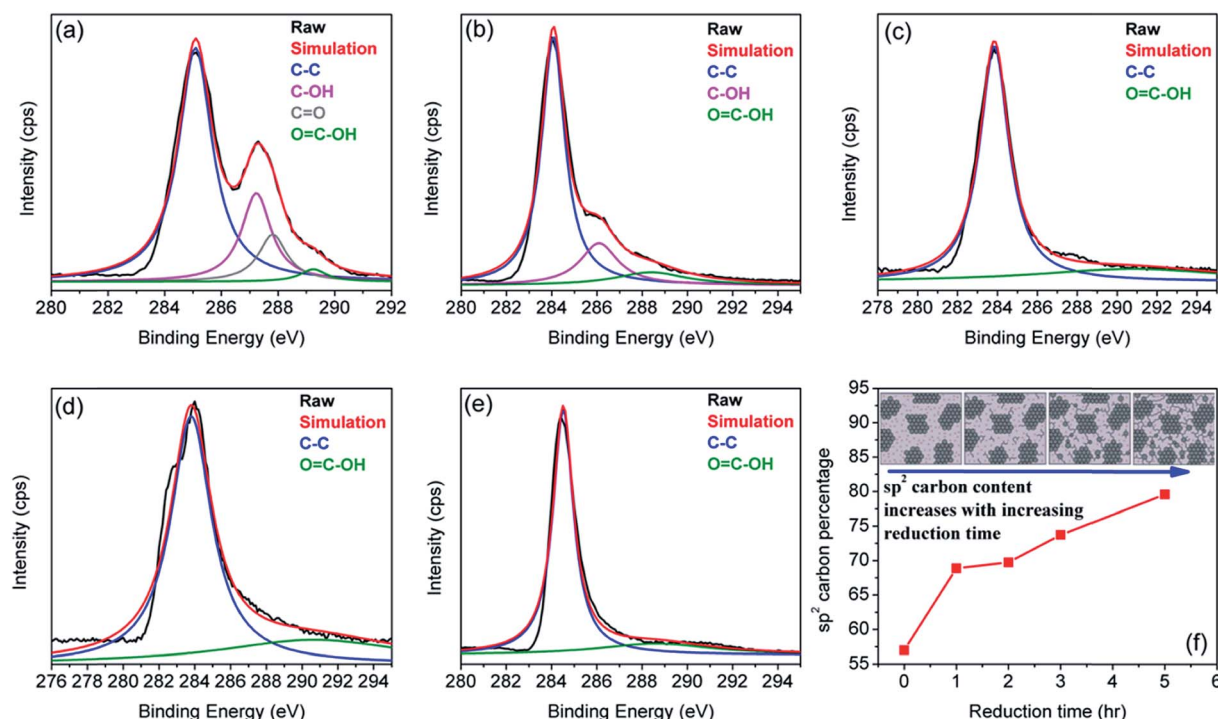
Fig. 1 XPS spectra of the rGO sample for (a) 0 h (GO), (b) 1 h, (c) 2 h, (d) 3 h, and (e) 5 h of reduction treatment. (f) Shows the variation of sp 2 carbon as a function of reduction time. The inset to (f) is a structural model of GO at various steps of the reduction process. Here, dark areas indicate sp 2 carbon domains, and light grey areas are sp 3 carbons consisting of oxygen groups (depicted as small dots). Reproduced with permission from ref. 18.
