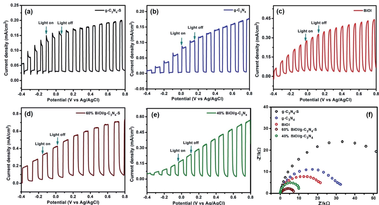
Fig. 5 Light on–off experiment for (a) pristine g-C 3 N 4 -S (b) pristine g-C 3 N 4 (c) pristine BiOI (d) g-C 3 N 4 -S/BiOI and (e) g-C 3 N 4 /BiOI; (f) Nyquist plots for the investigated samples obtained from EIS.
