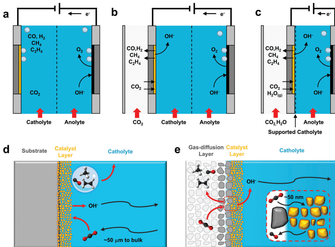
Fig. 2 Comparative mass transport phenomena in commonly-used electrochemical \text{CO}_2 reduction configurations. (a) Cell view for an H-cell configuration with a catalyst deposited on a solid substrate, (b) cell view for a catalyst deposited on a gas-diffusion layer with a flowing catholyte channel, (c) cell view for a catalyst deposited on a gas-diffusion layer with a non-flowing catholyte, (d) species transport to and from a catalyst layer in which \text{CO}_2 is supplied via diffusion from the bulk electrolyte on the microscale ( \sim 50 \mu\text{m} ). (e) A \text{CO}_2 reduction catalyst layer deposited onto a hydrophobic substrate with \text{CO}_2 diffusion from a nearby gas-liquid interface ( \sim 50 \text{nm} ). Liquid species diffuse to the ion-exchange membrane through either a bulk flowing electrolyte or a solid-supported electrolyte layer.
