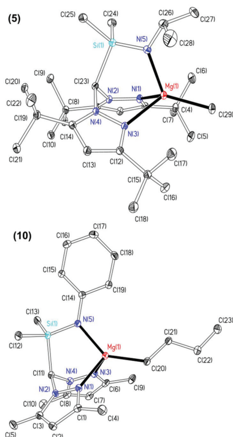
Fig. 1 Thermal displacement ellipsoid drawings (20% probability ellipsoids) of Mg{HC( t Bu 2 pz) 2 SiMe 2 NPr}Me ( 5 , top) and Mg{HC(Me 2 pz) 2 SiMe 2 NPh} n Bu ( 10 , bottom). All hydrogen atoms have been omitted for clarity.
