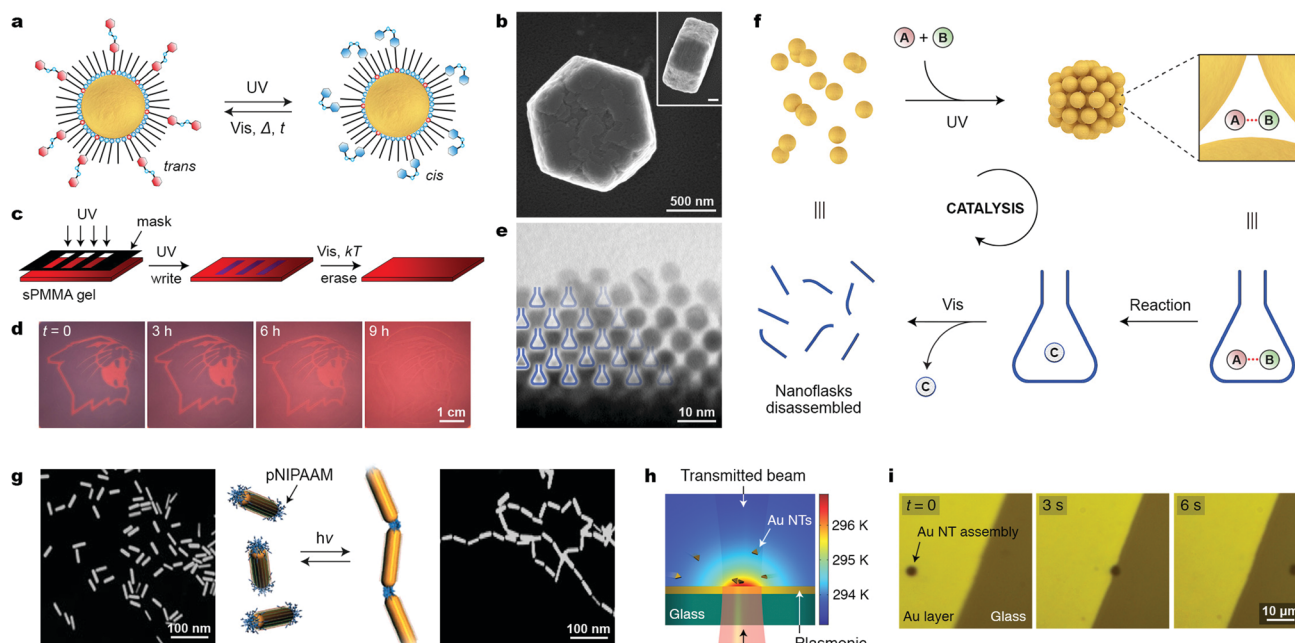
Fig. 10 Controlling the assembly of nanoparticles using light. (a) Photoinduced isomerization of azobenzene on a nanoparticle surface. The trans \rightarrow cis isomerization is accompanied by a large change in NP surface polarity and it can initiate the self-assembly process. (b) SEM image (top view) of a typical aggregate obtained from 5 nm Au NPs. The inset corresponds to a side view (scale bar, 200 nm). (c) Creating transient images using metastable NP aggregates as the “ink”. (d) Gradual (within 9 h) disappearance of an image accompanying the spontaneous disassembly of NP aggregates. (e) TEM image of an edge of a NP aggregate, whereby the nanopores between the NPs are represented as “nanoflasks”. (f) Schematic illustration of how the reversible formation of nanopores within NP aggregates can accelerate a chemical reaction. (g) Light-controlled collapse of thermoresponsive polymers at the tips of gold nanorods drives their self-assembly. (h) Self-assembly of gold nanotriangles (NTs) driven by light-induced thermophoresis. (i) Light-controlled stabilization and long-distance optical manipulation of an ensemble of Au NTs. Adapted with permission from ref. 60 (copyright 2016, Nature Publishing Group) (b, e and f), ref. 68 (copyright 2009, Wiley-VCH) (c and d), ref. 65 (copyright 2009, Royal Society of Chemistry) (g), and ref. 67 (copyright 2016, American Chemical Society) (h and i).
