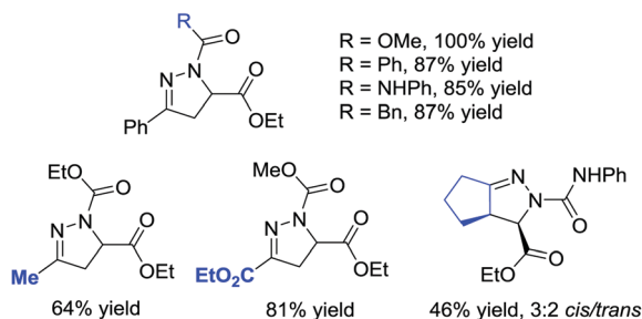
Scheme 3 Cu(II)-Catalyzed formal [4+1] annulation of diazo compounds with in situ generated azoalkenes.
