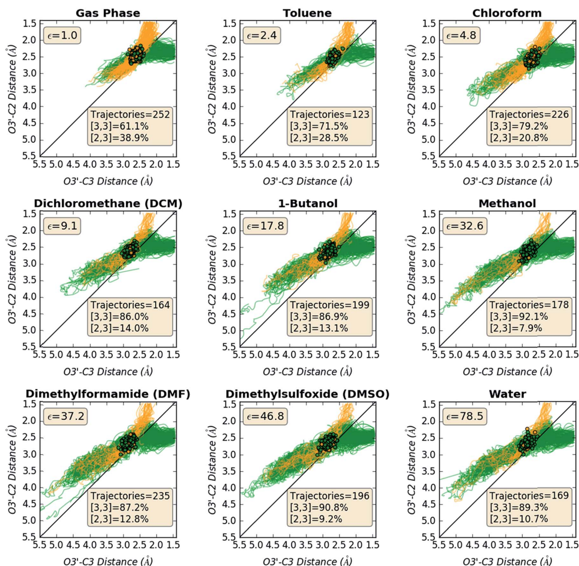
Fig. 7 Paths of trajectories, with respect to \text{O3}'\text{-C2} and \text{O3}'\text{-C3} distances. The plots show the starting points (clustered points) of all trajectories for each system and their geometric changes along the trajectories colored by the product made: yellow-orange for [2,3] product (top region of the graphs, where the \text{O3}'\text{-C2} distance is small) and green for [3,3] product (top right region of the graphs, where the \text{O3}'\text{-C3} distance is small). The bottom left region of the graphs corresponds to the reactant side of the trajectories.
