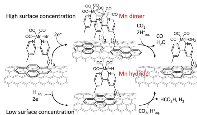
Scheme 10 Two-electron reduction of \text{CO}_2 to CO vs. \text{HCOOH} with the [\text{MnBr}(2,2'\text{-bipyridine})(\text{CO})_3] complex anchored to a carbon nanotube electrode via a pyrene unit depending on the surface concentration. Reprinted with permission from ref. 134. Copyright 2017, American Chemical Society.
