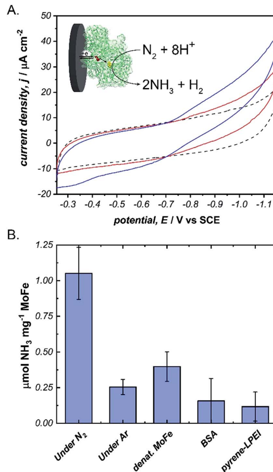
Fig. 4 (A) Cyclic voltammograms of pyrene-LPEI films containing MoFe protein and 5 mg mL -1 MWCNT-COOH under Ar (---), and after 5 min (—), or 10 min (—) of bubbling ultra high purity \text{N}_2 . (B) Production of \text{NH}_3 using \text{N}_2 as the only substrate after constant potential bulk electrolysis of pyrene-LPEI/MoFe films for 8 h. CVs were performed using 100 mM MOPS buffer at pH 7.0, 25 °C and a scan rate of 5 mV s -1 . Bulk electrolysis was performed using 100 mM MOPS buffer pH 7.0 at -1.1 V vs. SCE and 25 °C. Error bars represent one standard deviation, where n = 3 .
