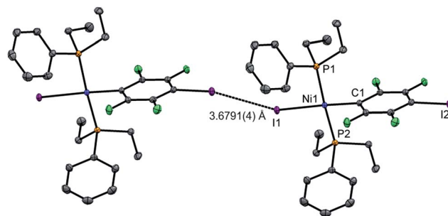
Fig. 2 Molecular structure of 2pl showing intermolecular C-I\cdots I halogen bond. Displacement ellipsoids at 50% probability level. Hydrogen atoms not shown. A three-molecule chain is illustrated in the ESI.†
